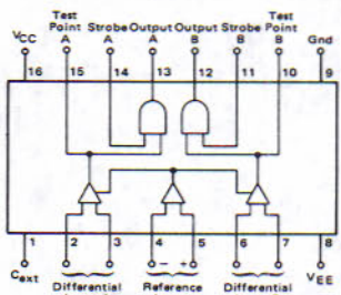
MC5528 MC5529 -55 to 125°C L Suffix — Case 620
