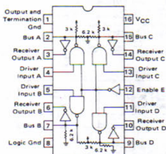
MC3441 0 to 70°C P Suffix — Case 648 Quad Transceivers with all four drivers controlled by a Common-Enable Input R1 = 3.0 k (to V_{CC} ) R2 = 6.2 k (to Gnd)
