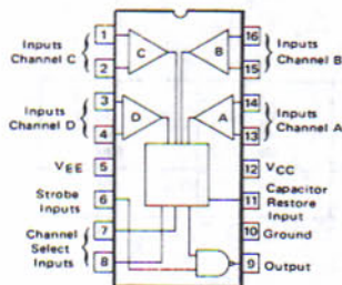
MC1544 -55 to 125°C L Suffix — Case 620 F Suffix — Case 650
