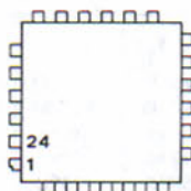
BEAM LEAD CHIP (24 Lead) (Geometry Side Down)
