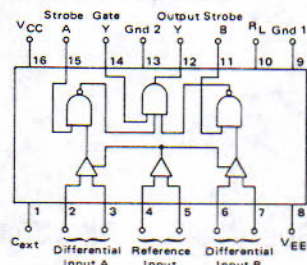
MC5522 MC7522 -55 to 125°C L Suffix — Case 620
