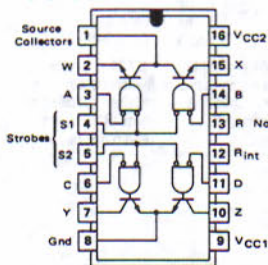
MC5532 -55 to 125°C L Suffix — Case 620 F Suffix — Case 650
